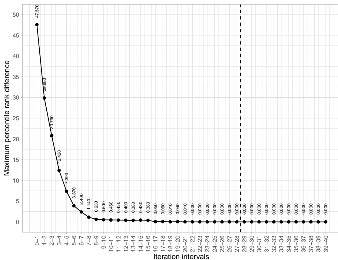
Figure 2: Maximum percentile ranks variation between iterations
